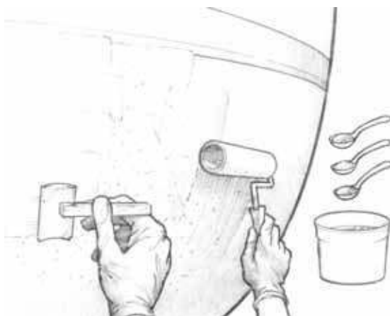
Figure 7.4. Add 422 Barrier Cat Additive to the second and remaining coats to increase moisture exclusion effectiveness and abrasion resistance.
